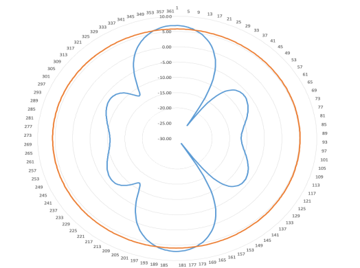
5.5 GHz Radiation Pattern
