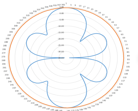
2.45 GHz Radiation Pattern
